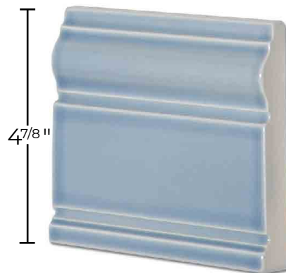
Ogee Base OG-BAS1 Group C Corners: IP, LP, RP
