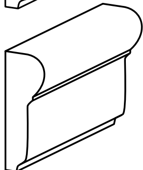
SBB Mud Cap SB-MUD1 Group C Corners: IP, LP, RP 3 1/8" H x 6" L x 1" D
