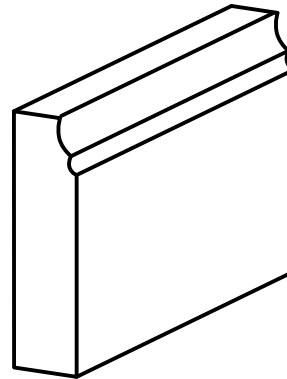
Plaza Base C PL-BSC1 Group C Corners: IP, LP, RP 3 1/8" H x 6" L x 7/8" D
