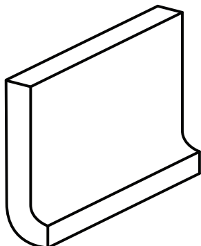
4x6 Cove Base ST-C461 Group B Corners: IC, OC, LP, RP 4" H x 6" L x 3/4" D
