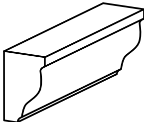
Plaza Rail PL-RAI1 Group B Corners: DA, UA, IC, OC, LP, RP 1 1/2" H x 6" L x 1" D
