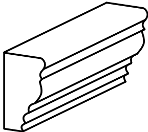
Small Plaza PL-PLS1 Group B Corners: DA, UA, IC, OC, LP, RP 2" H x 6" L x 1" D
