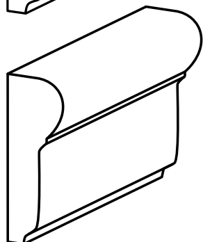
SBB Mud Cap SB-MUD1 Group C Corners: IP, LP, RP 3 1/8" H x 6" L x 1" D
