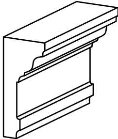
Plaza Cap PL-CAP1 Group C Corners: DA, UA, IP, LP, RP 3 3/8" H x 6" L x 1 1/2" D
