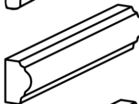
Ogee Ridge OG-RID1 Group A Corners: DA, UA, IC, OC, RP, LP 1" H x 6" L x 5/8" D
