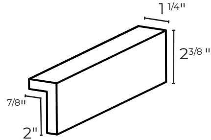
Long 90° Angle ST-90L1 Group B Corners: OC
