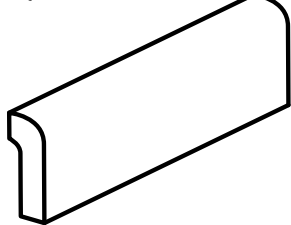
Radius Bullnose ST-R261 Group B Corners: DA, UA, IC, OC 1 7/8" H x 6" L x 7/8" D
