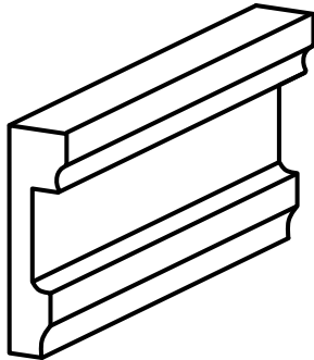
Plaza Ogee PL-OGE1 Group B Corners: DA, UA, IC, OC, LP, RP 2 1/2" H x 6" L x 7/8" D
