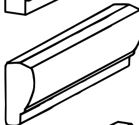
Rail ST-RAI1 Group B Corners: DA, UA, IC, OC, RP, LP 1 1/2" H x 6" L x 7/8" D
