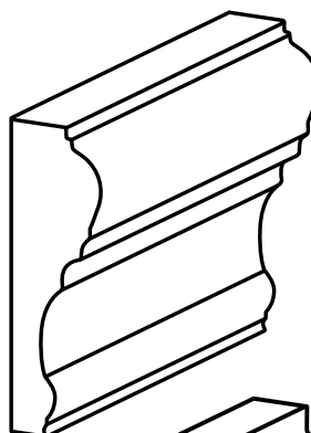
Ogee Cap OG-CAP1 Group C Corners: IP, LP, RP 4 5/8" H x 6" L x 1 1/2" D
