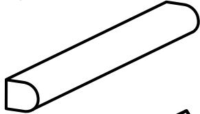
HRA HR-HRA1 Group B Corners: DA, IC, OC, LP 1 1/8" H x 6" L x 3/4" D
