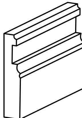
Plaza Base B PL-BSB1 Group C Corners: IP, LP, RP 4 3/4" H x 6" L x 7/8" D
